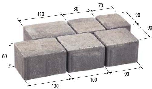
Layout dimensions, set of 6 types of stones
