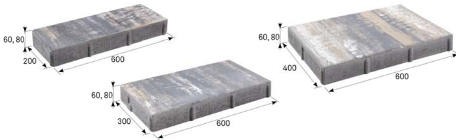
Layout dimensions, set of 3 types of stones
