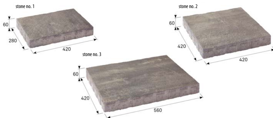
Layout dimensions, set of 3 types of stones
