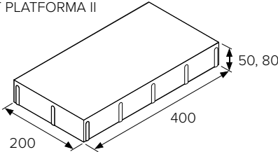
BEST PLATFORMA II
