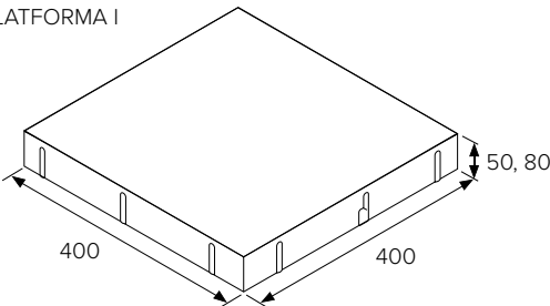
BEST PLATFORMA I
