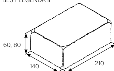
BEST LEGENDA II
